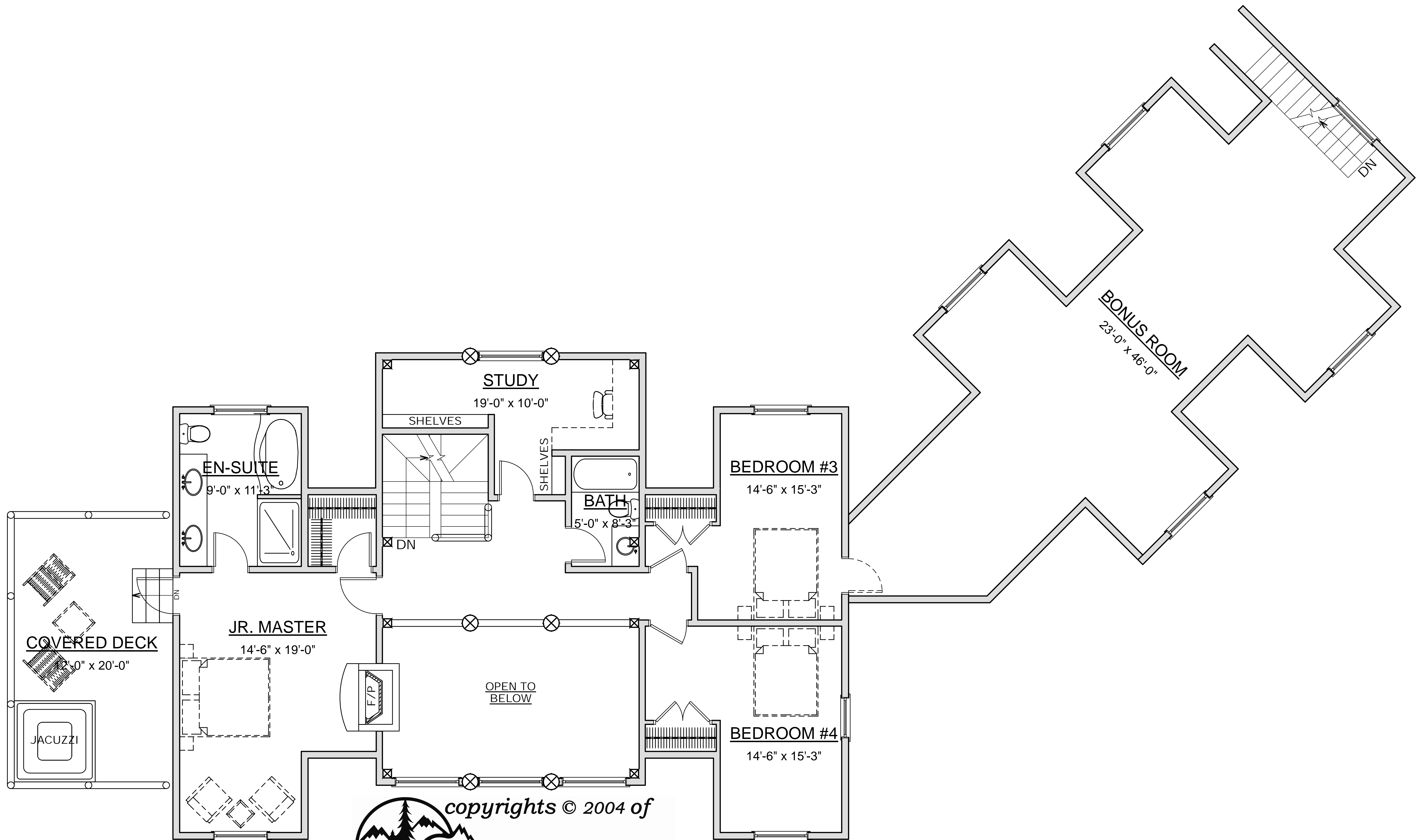
UPPER FLOOR PLAN AREA: 1,190 SQ.FT.
