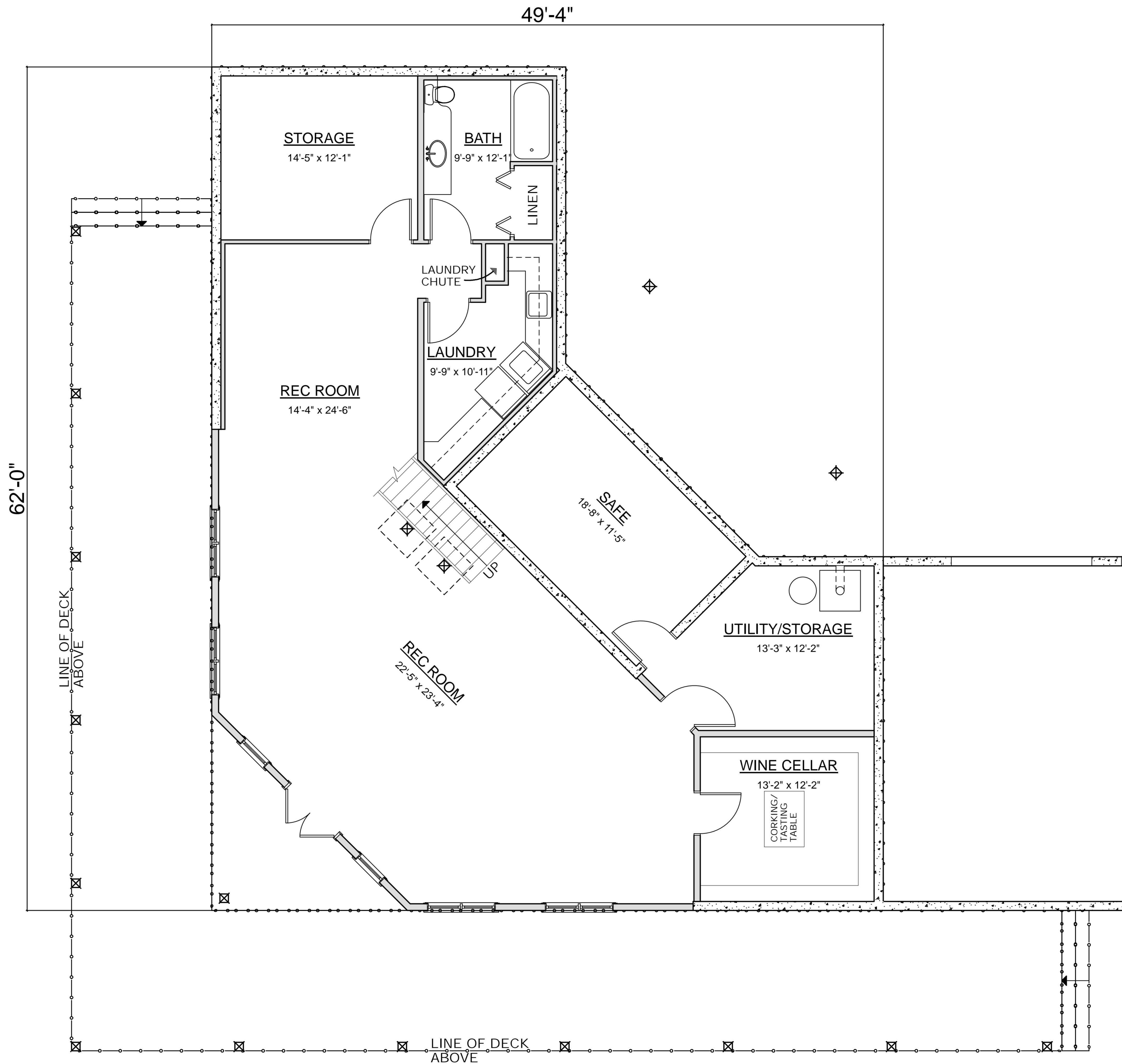
BASEMENT FLOOR PLAN AREA: 2,225 SQ. FT.
