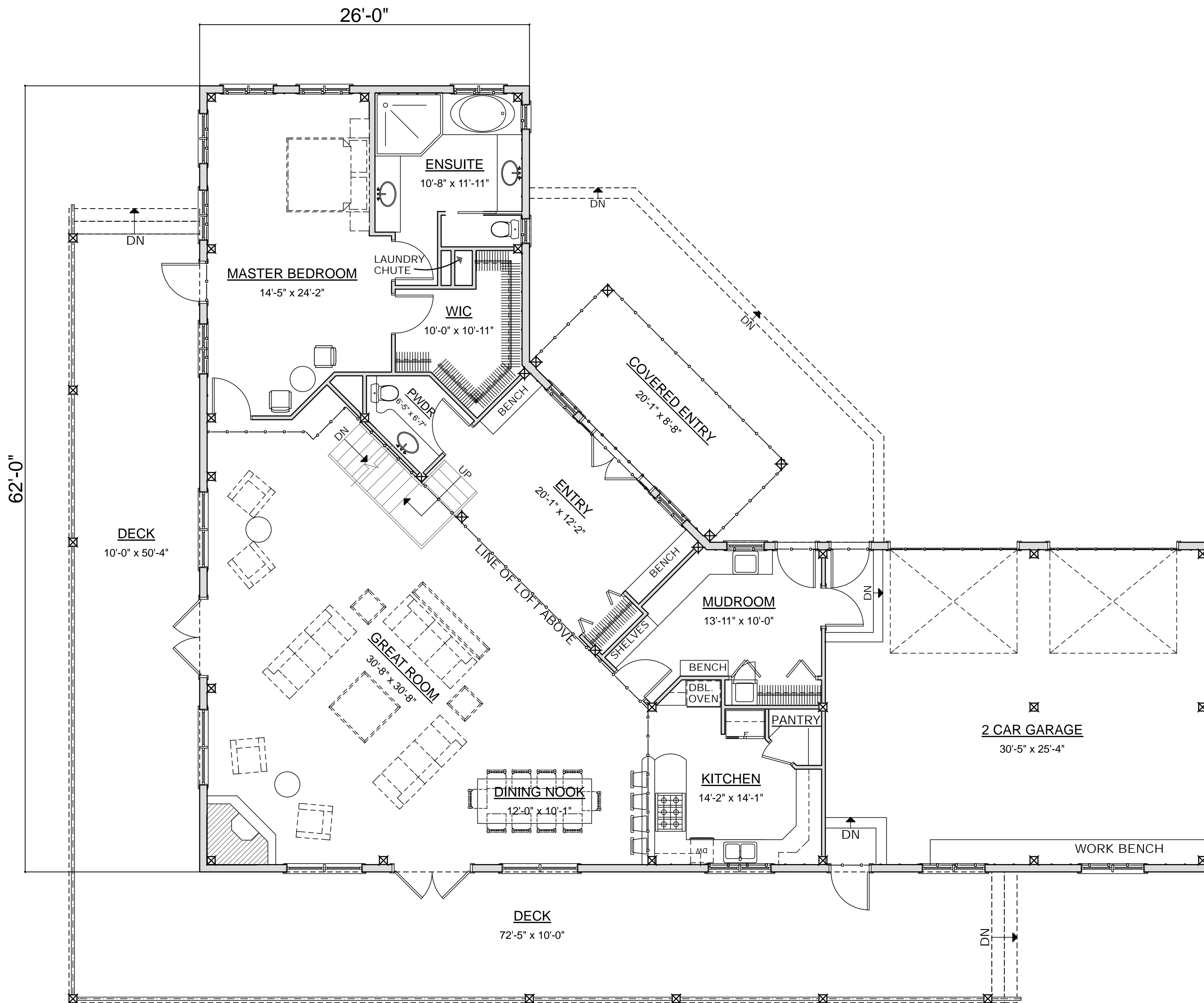
FIRST FLOOR PLAN AREA: 2,318 SQ.FT.
