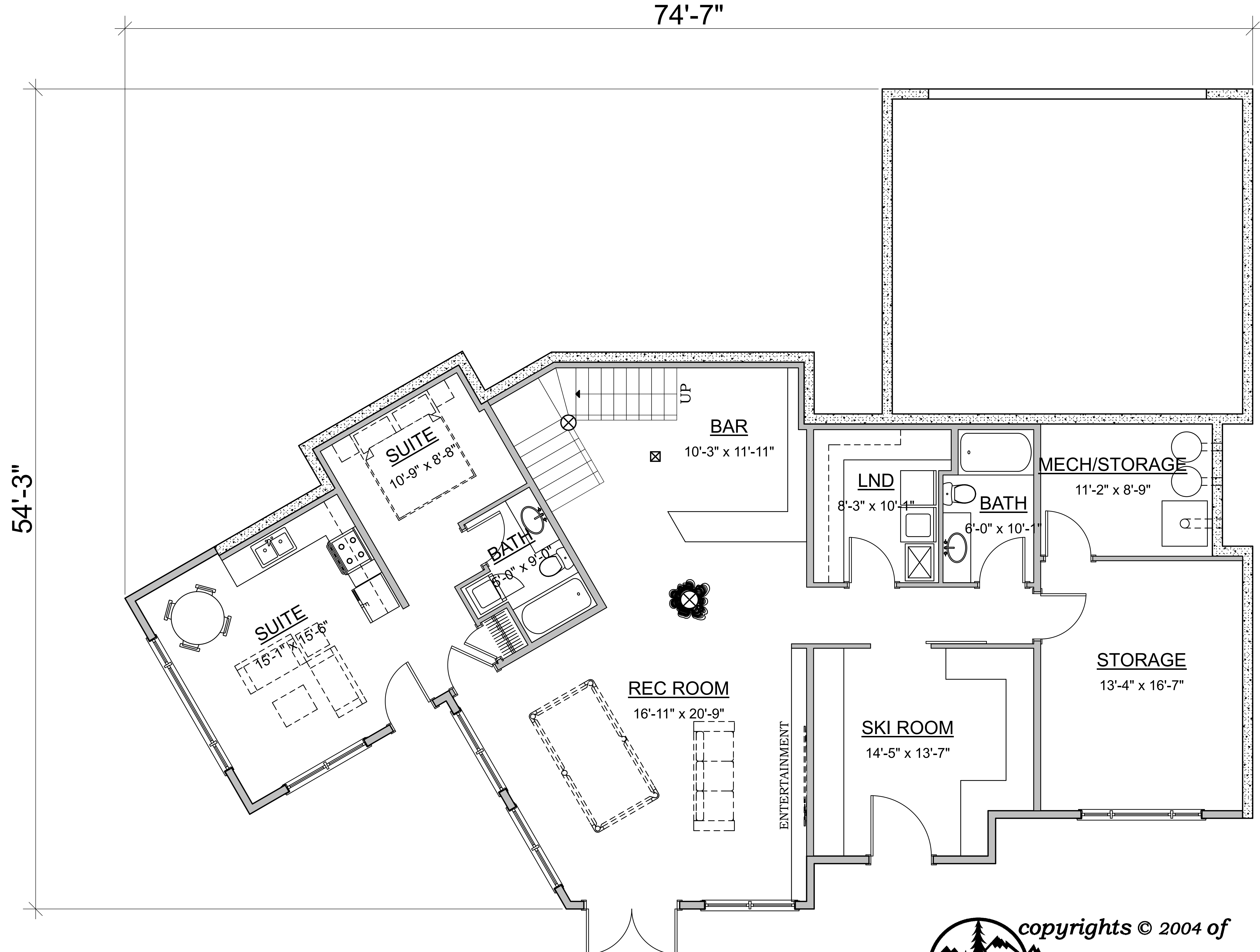
BASEMENT PLAN AREA: 1,985.90 sq ft
