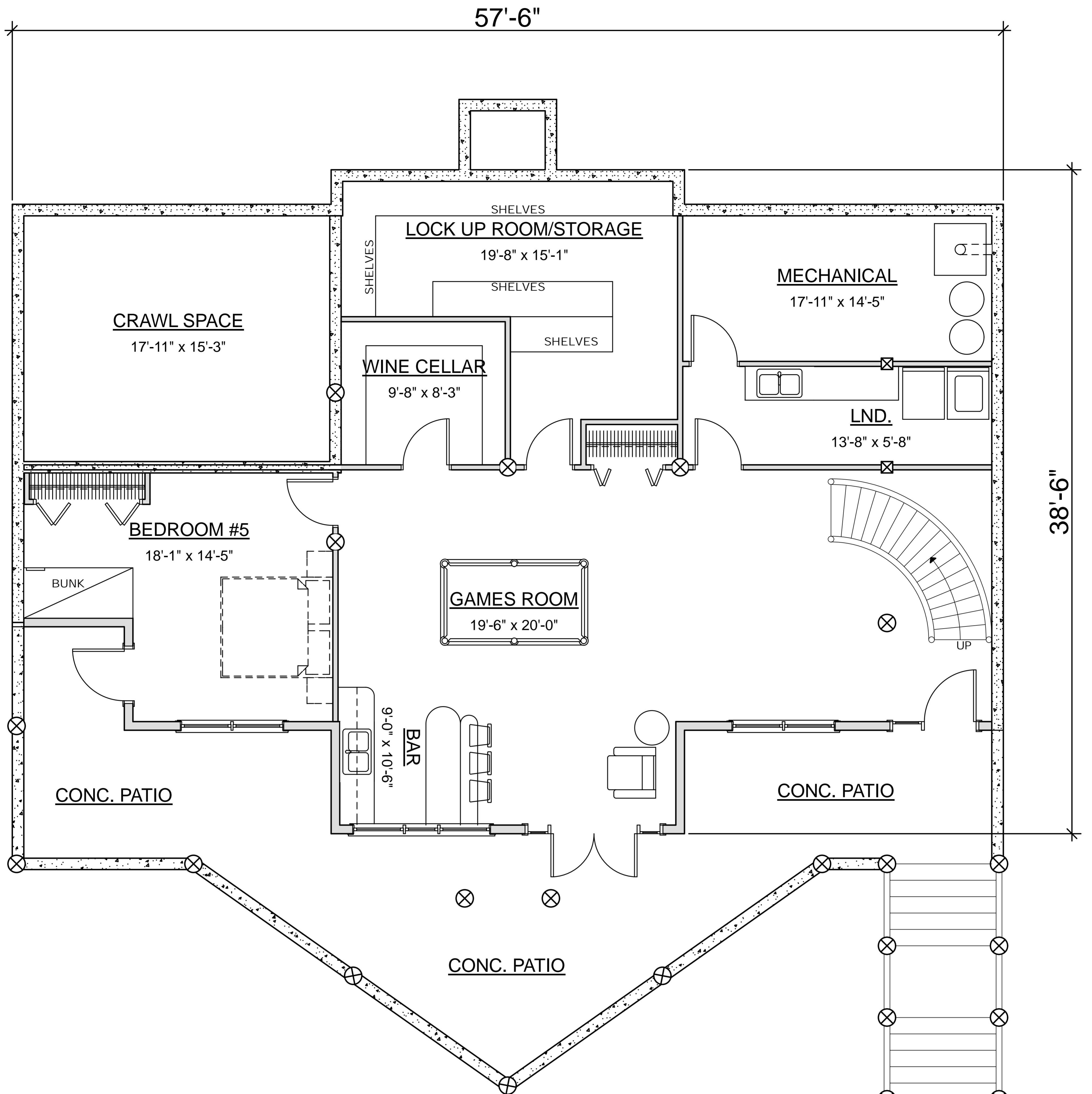
BASEMENT FLOOR PLAN AREA: 1,600 SQ. FT.
