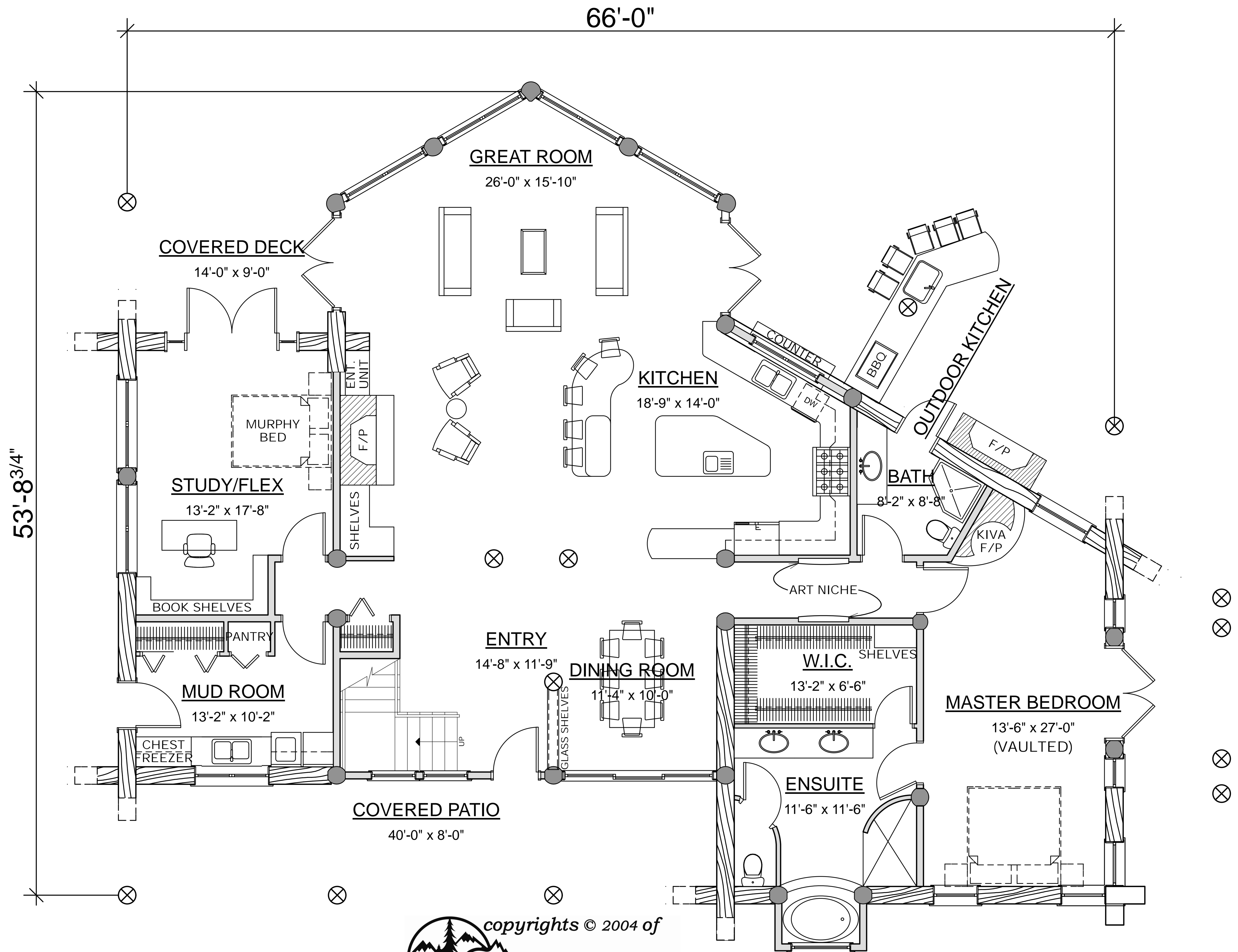
MAIN FLOOR PLAN AREA: 2,373 SQ. FT.
