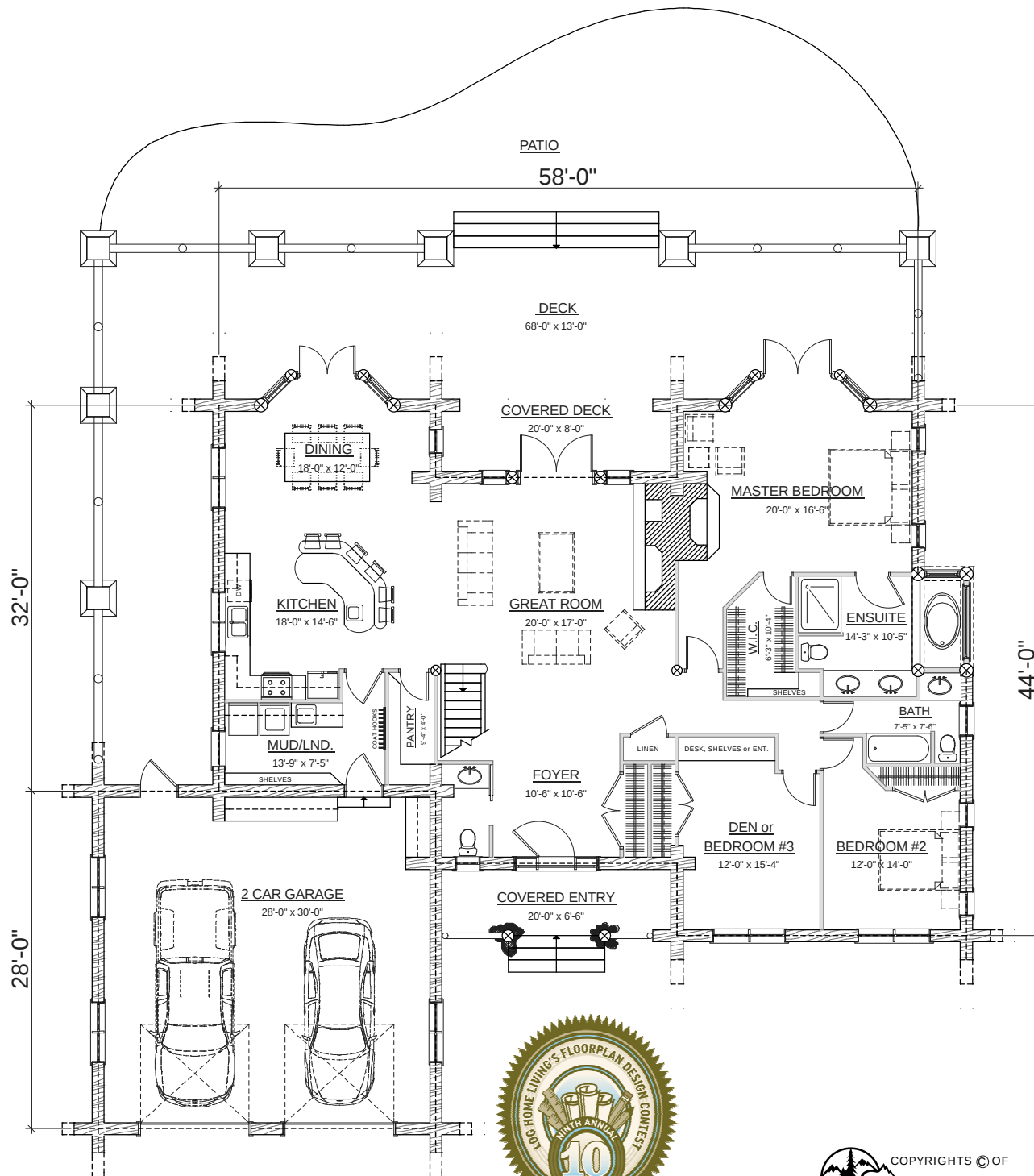
FIRST FLOOR PLAN AREA: 2210 SQ.FT.
