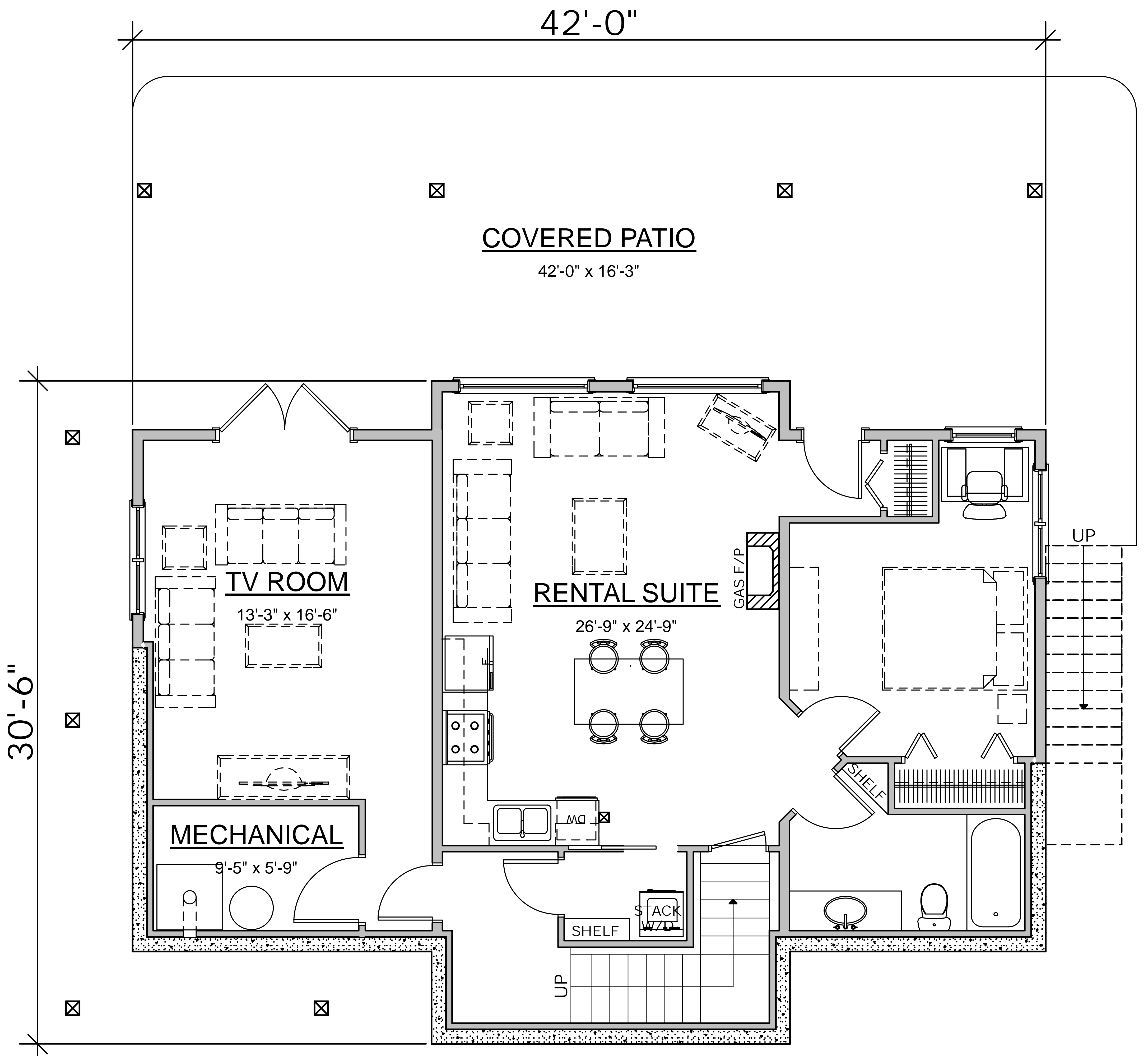
BASEMENT FLOOR PLAN AREA: 1061 SQ. FT.
