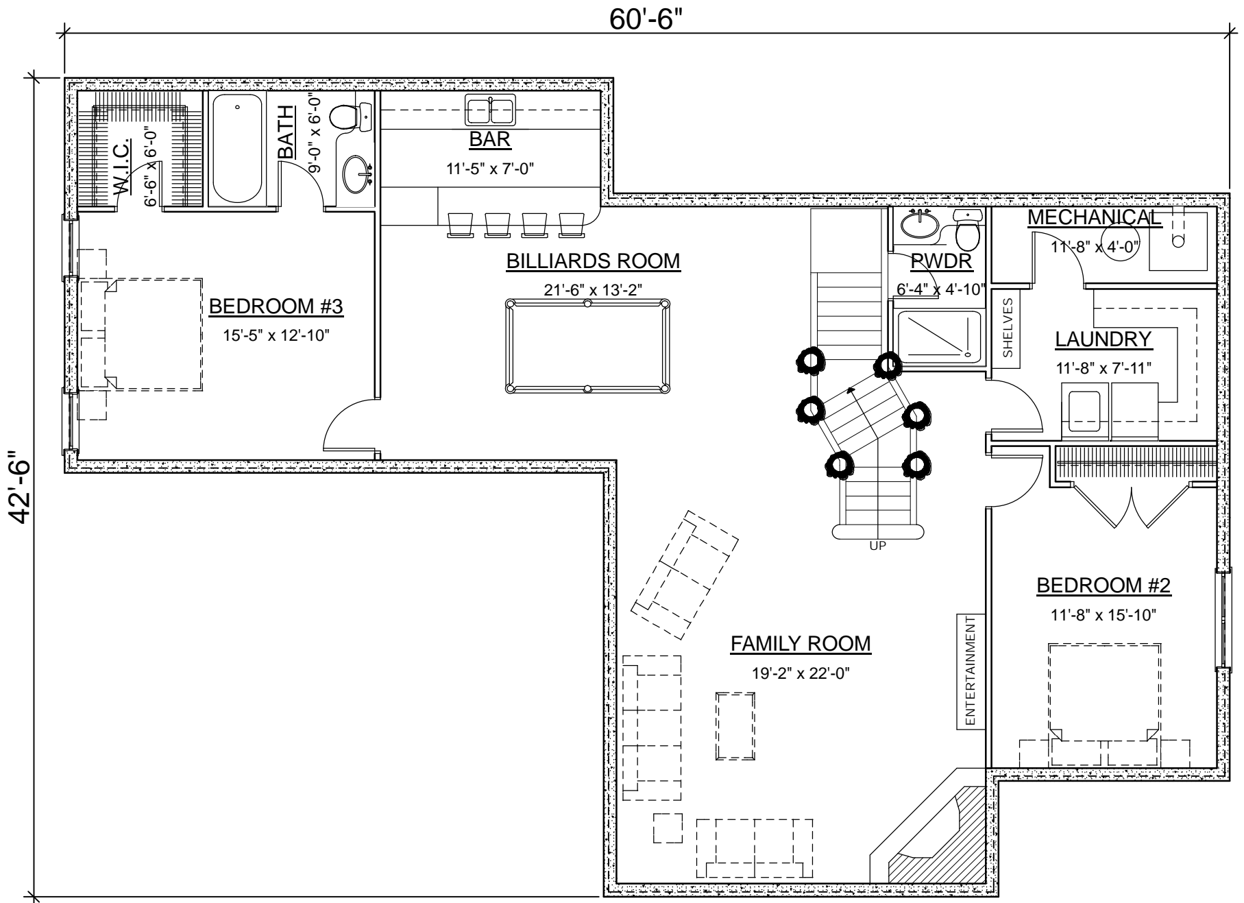
BASEMENT FLOOR PLAN AREA: 1690 SQ. FT.
