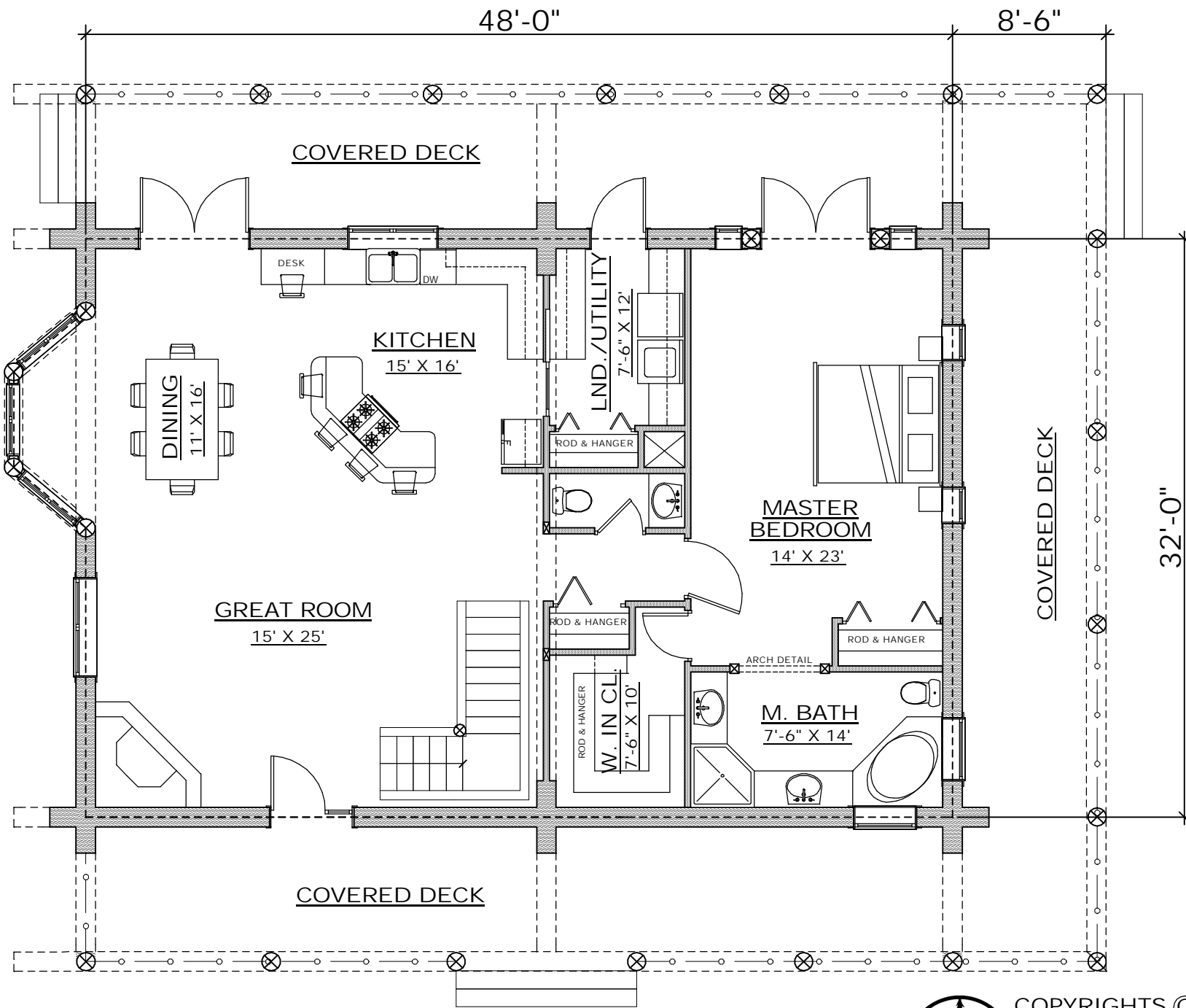
FIRST FLOOR PLAN AREA: 1600 SQ.FT.
