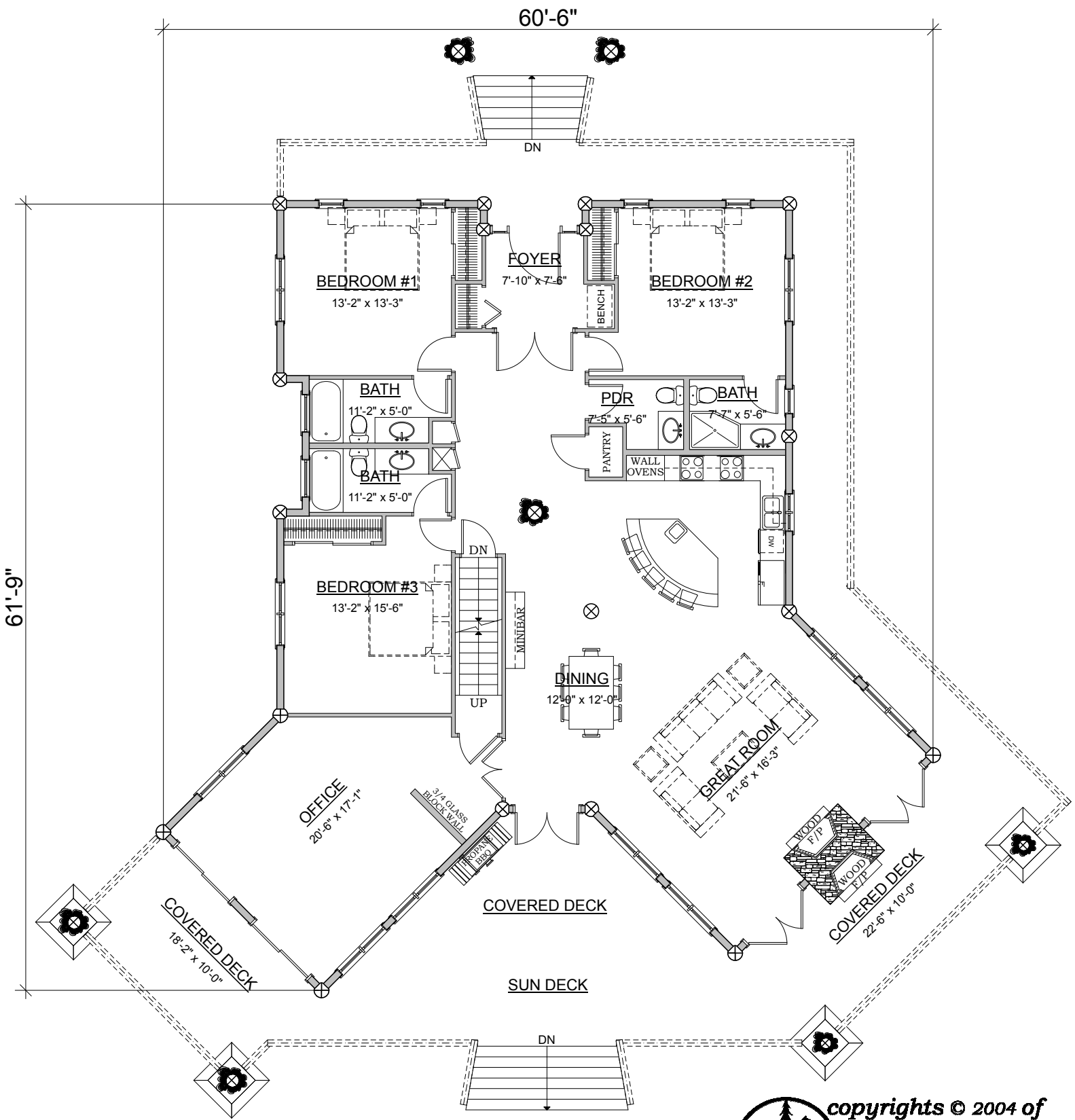
FIRST FLOOR PLAN AREA: 2386 SQ. FT.
