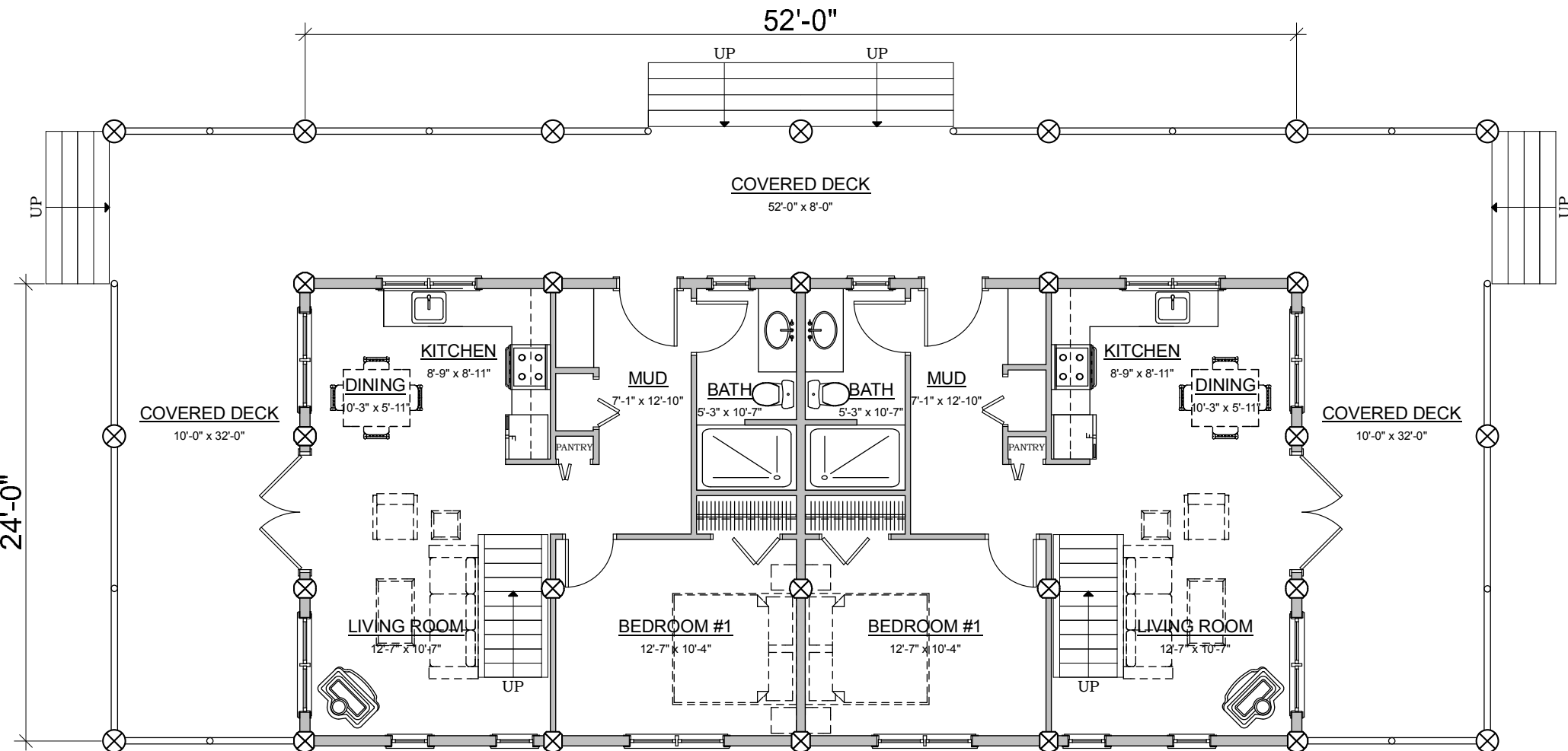
FIRST FLOOR PLAN TOTAL AREA: 1286 SQ.FT.
