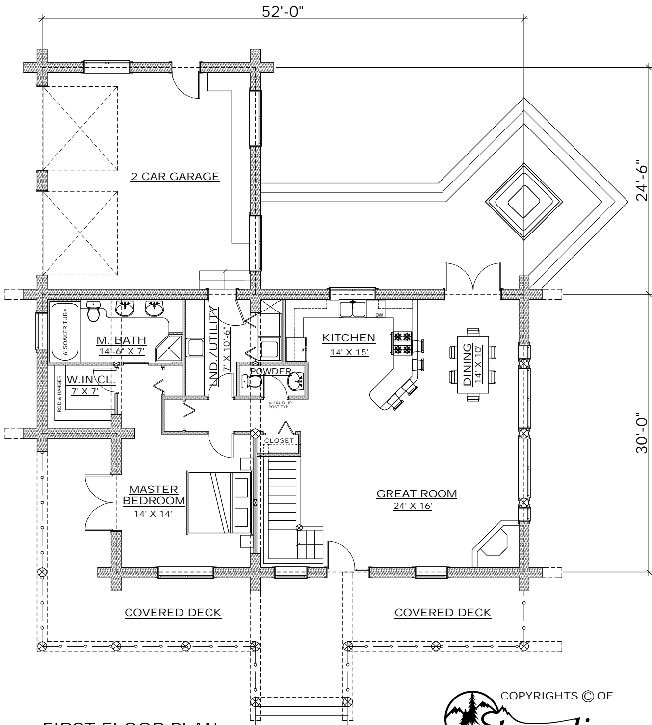
FIRST FLOOR PLAN AREA: 1740 SQ. FT.
