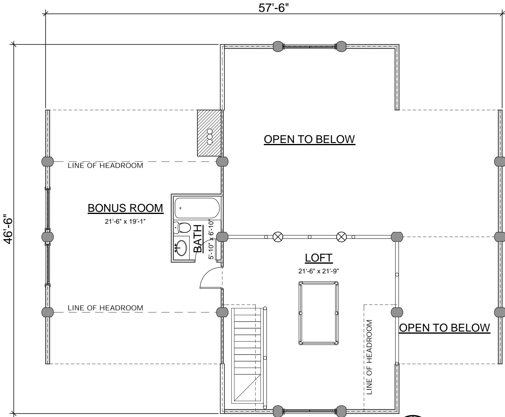
SECOND FLOOR PLAN AREA: 915 SQ. FT.
