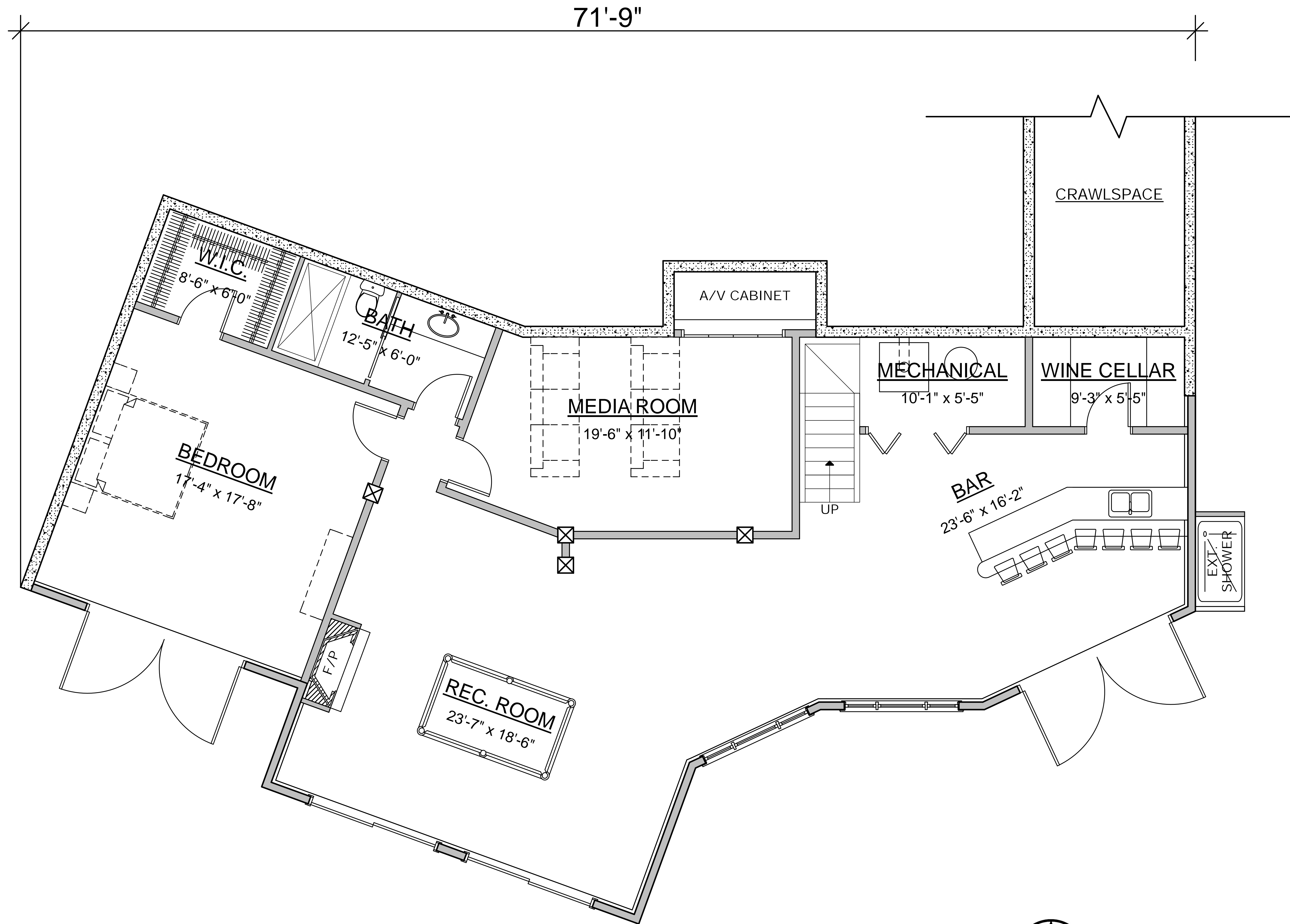
BASEMENT FLOOR PLAN AREA: 1936 SQ.FT.
