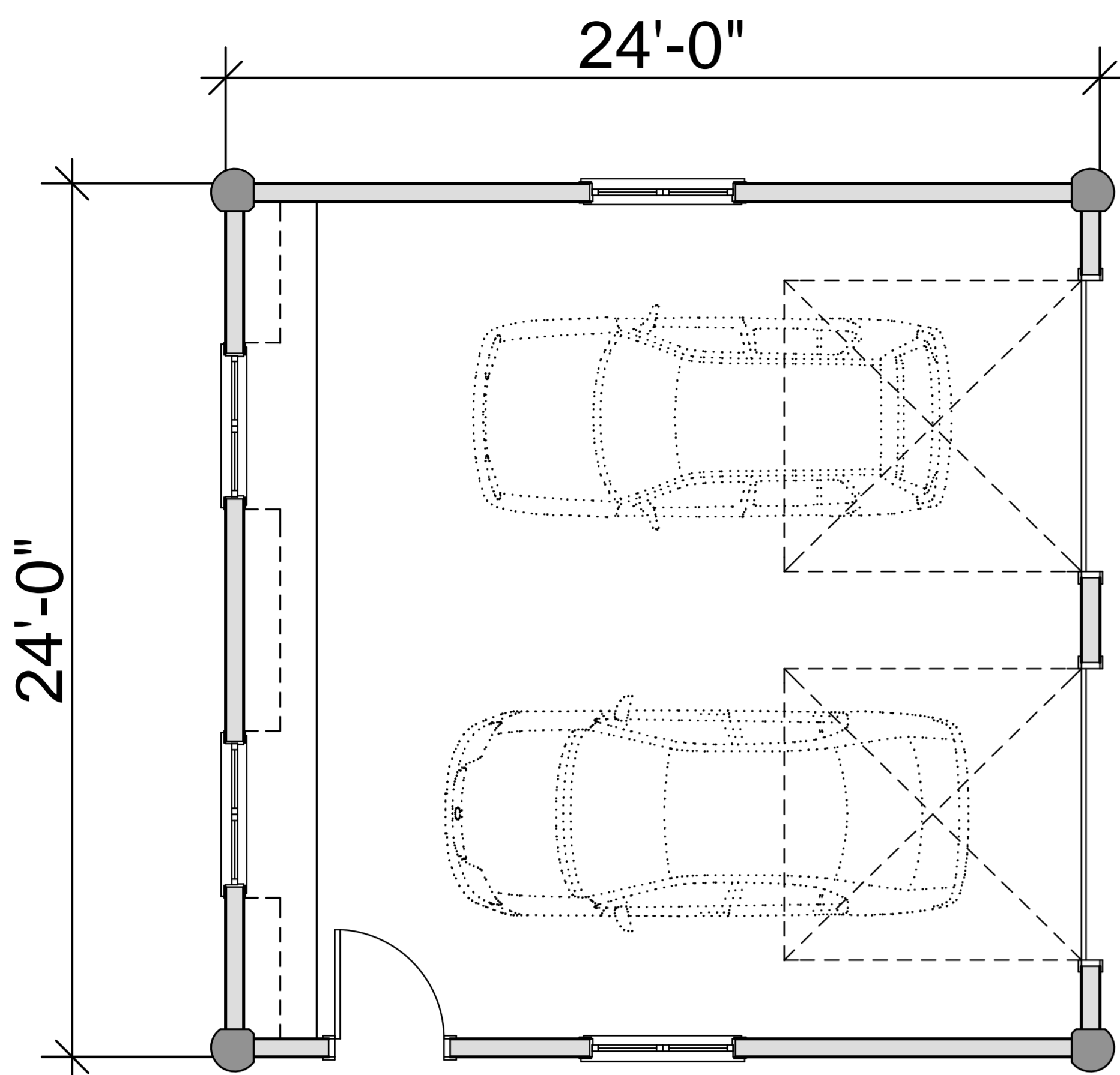
GARAGE FLOOR PLAN AREA: 576 SQ.FT.
