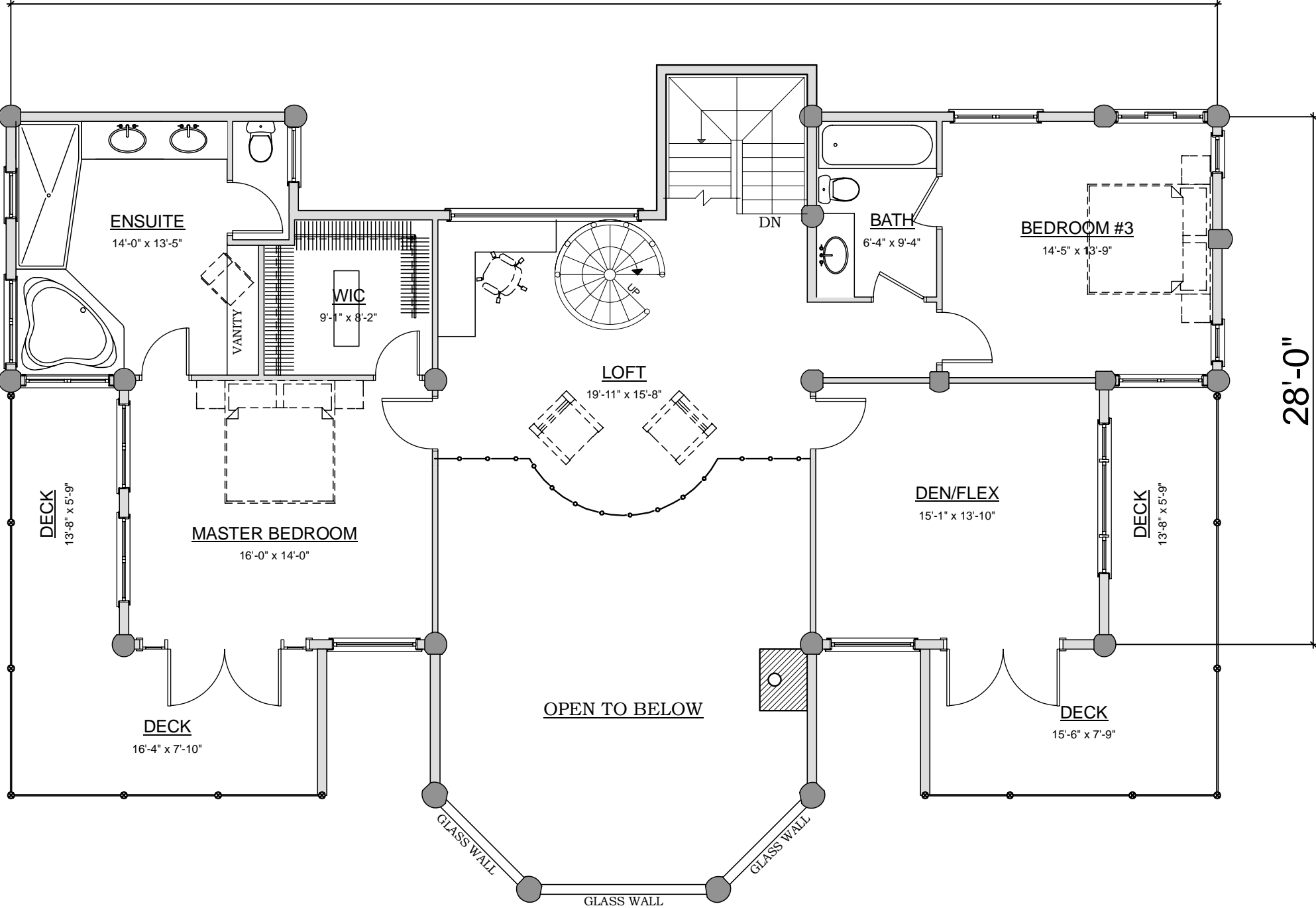
SECOND FLOOR PLAN AREA: 1,340 SQ. FT.
