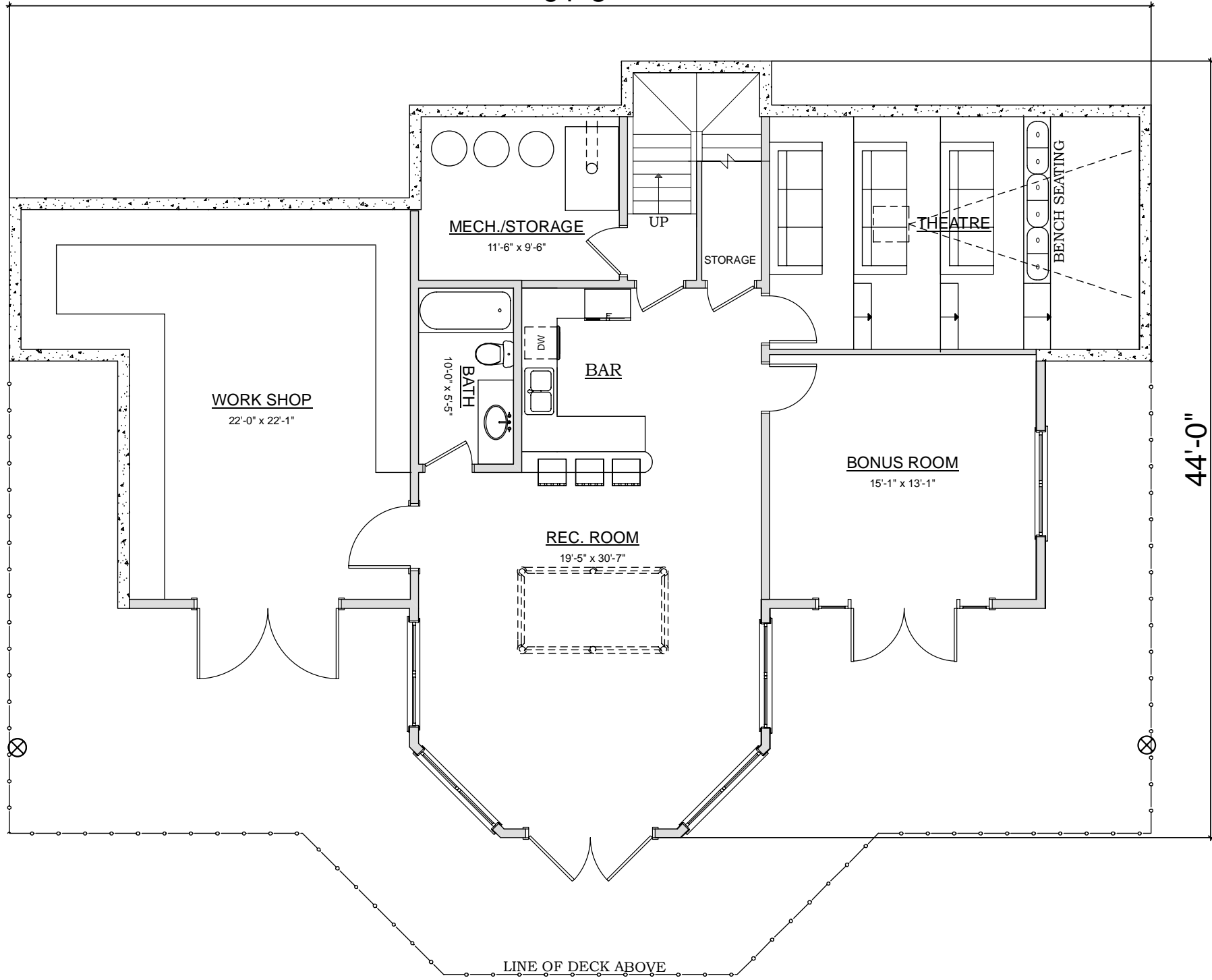
BASEMENT PLAN AREA: 1,821 SQ. FT.
