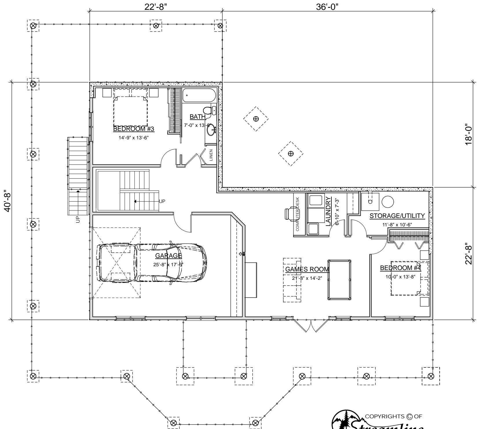
BASEMENT FLOOR PLAN AREA: 1,250 SQ. FT. GARAGE: 485 SQ.FT.
