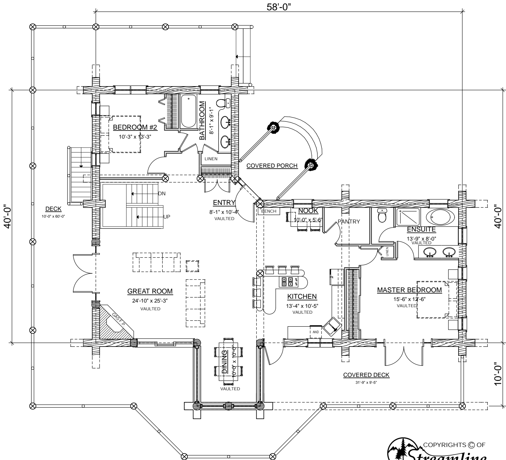
FIRST FLOOR PLAN AREA: 1845 SQ.FT.
