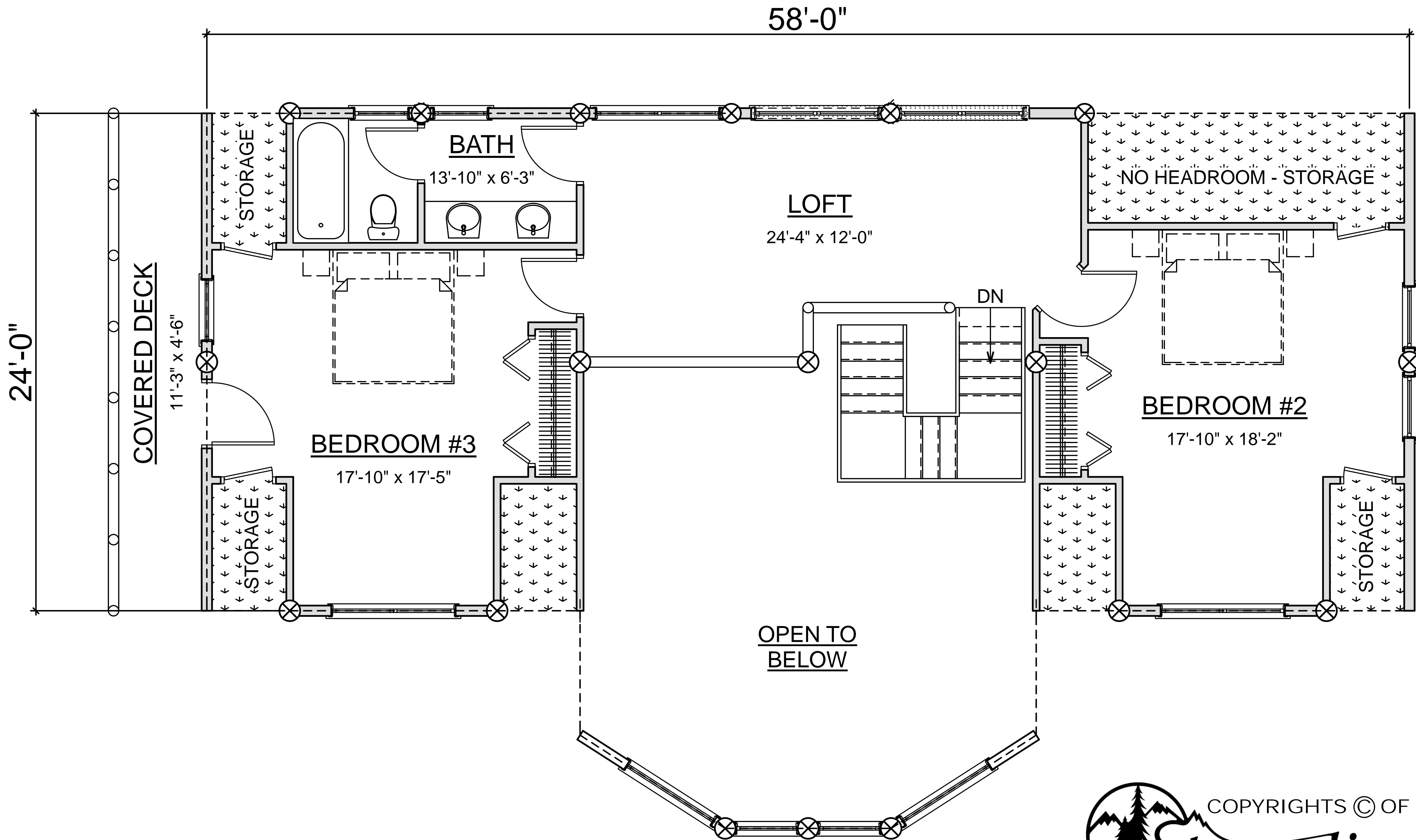
SECOND FLOOR PLAN AREA: 845 SQ. FT.
