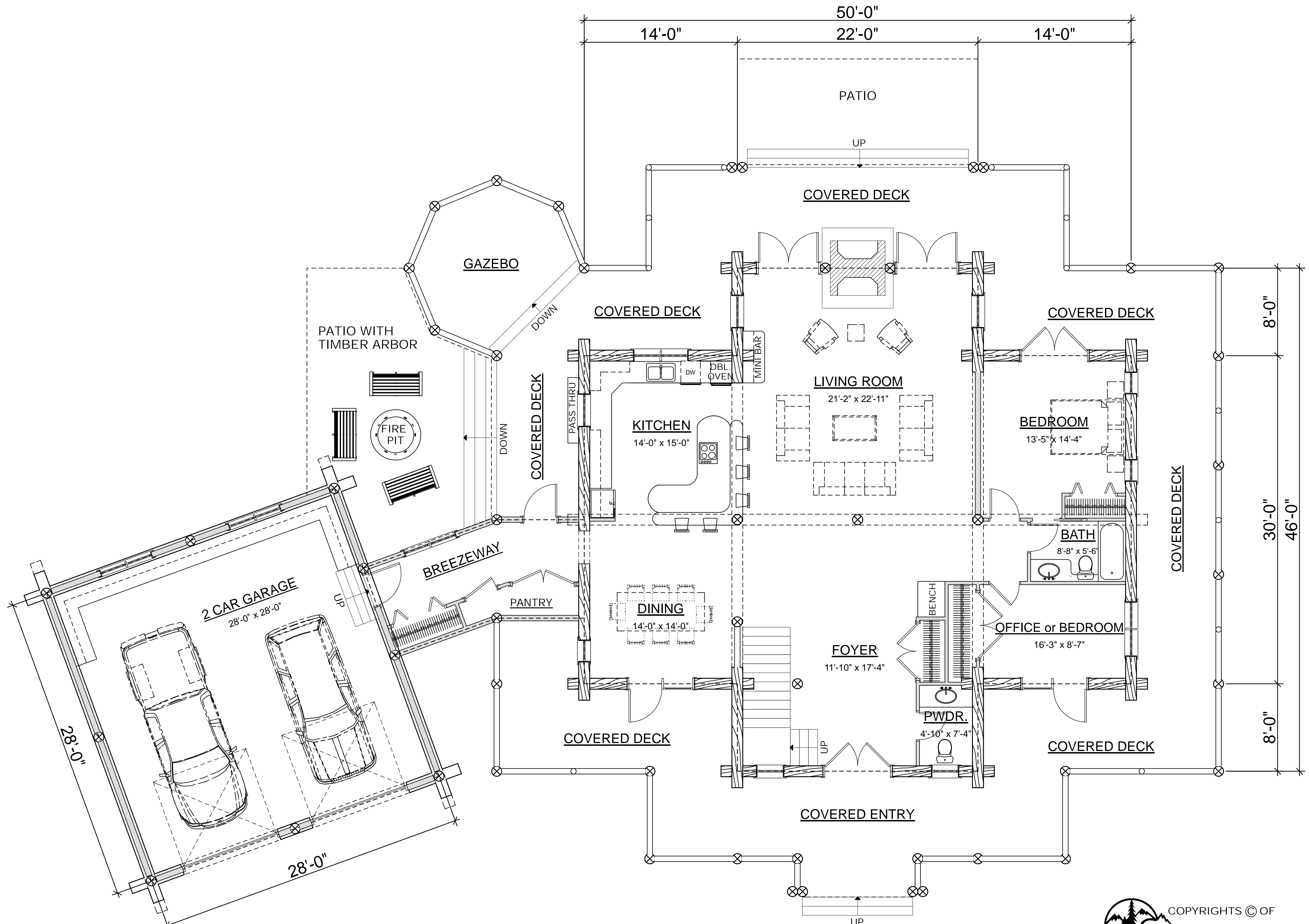
FIRST FLOOR PLAN AREA: 2,090 SQ. FT.
