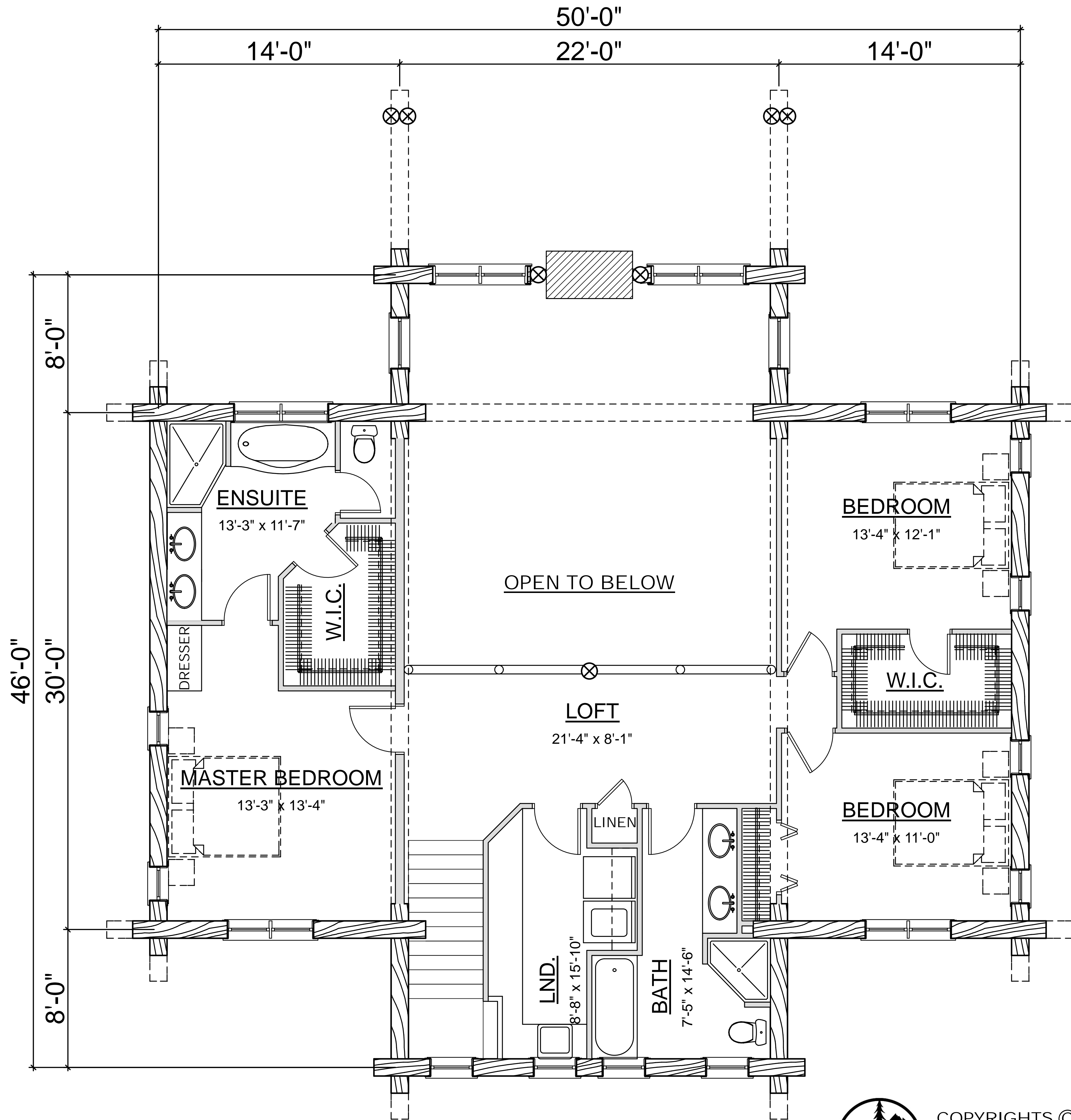
SECOND FLOOR PLAN AREA: 1,280 SQ. FT.
