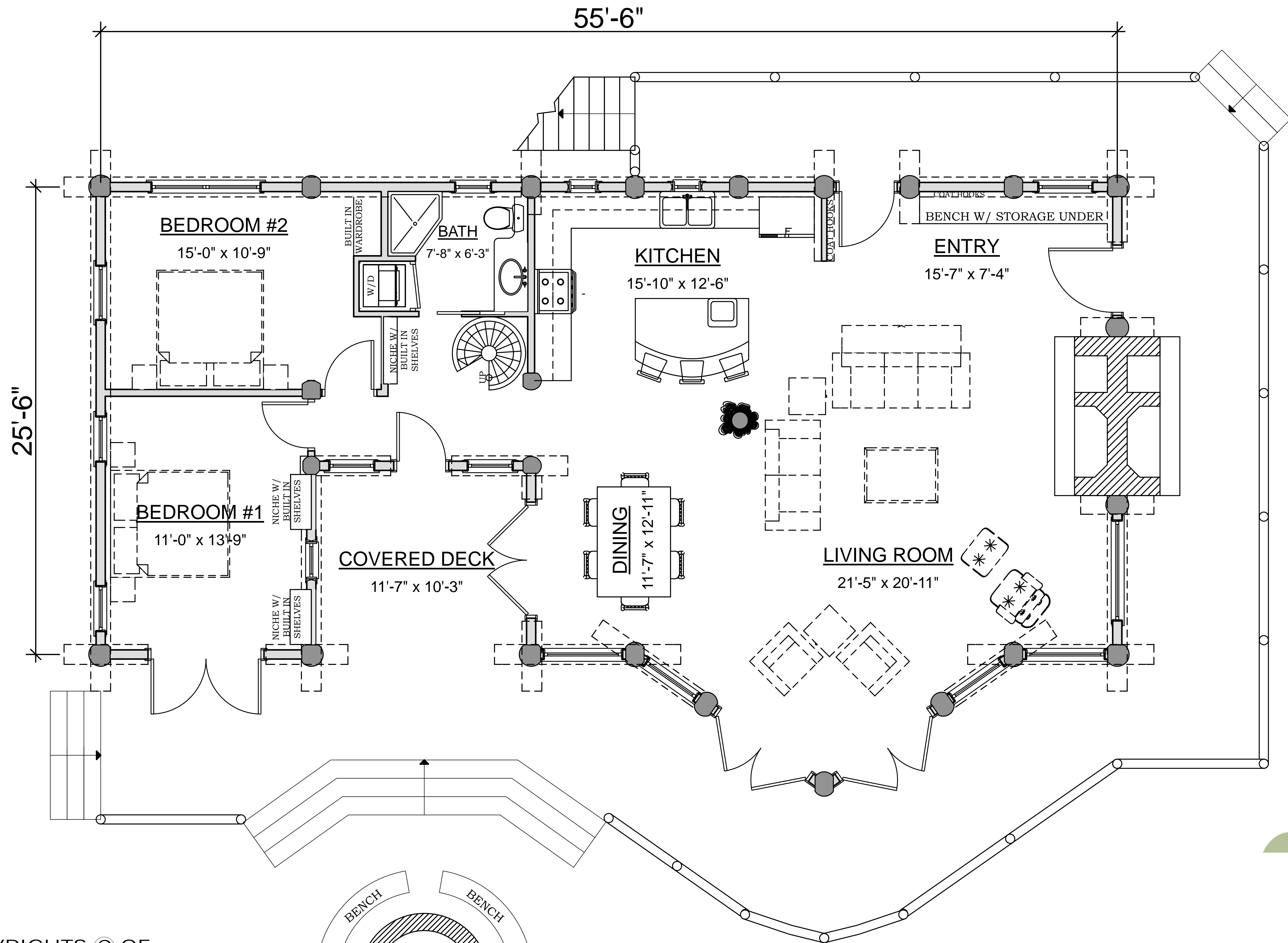
FIRST FLOOR PLAN AREA: 1410 SQ.FT.
