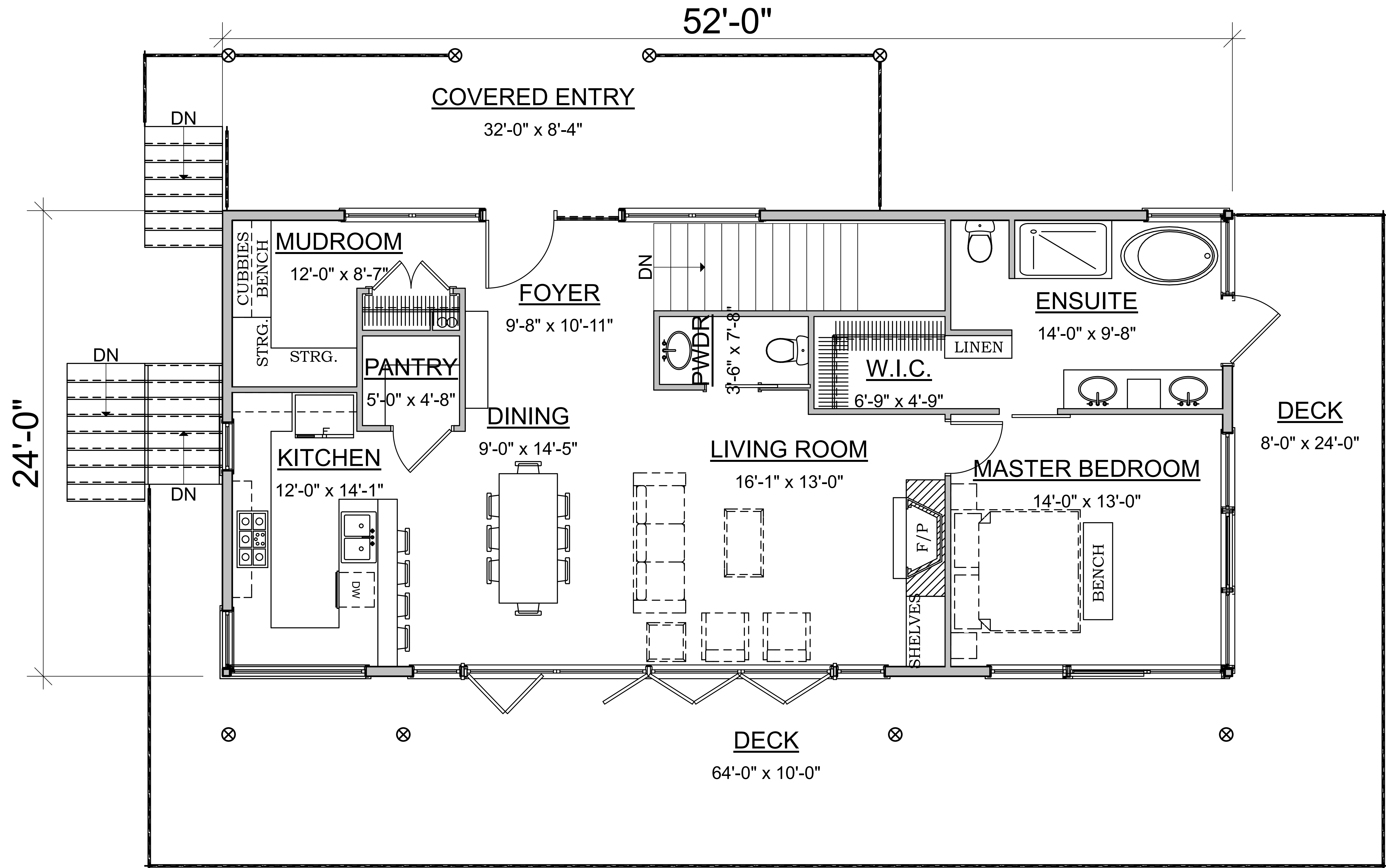
FIRST FLOOR PLAN MAIN FLOOR AREA: 1,178 sq ft
