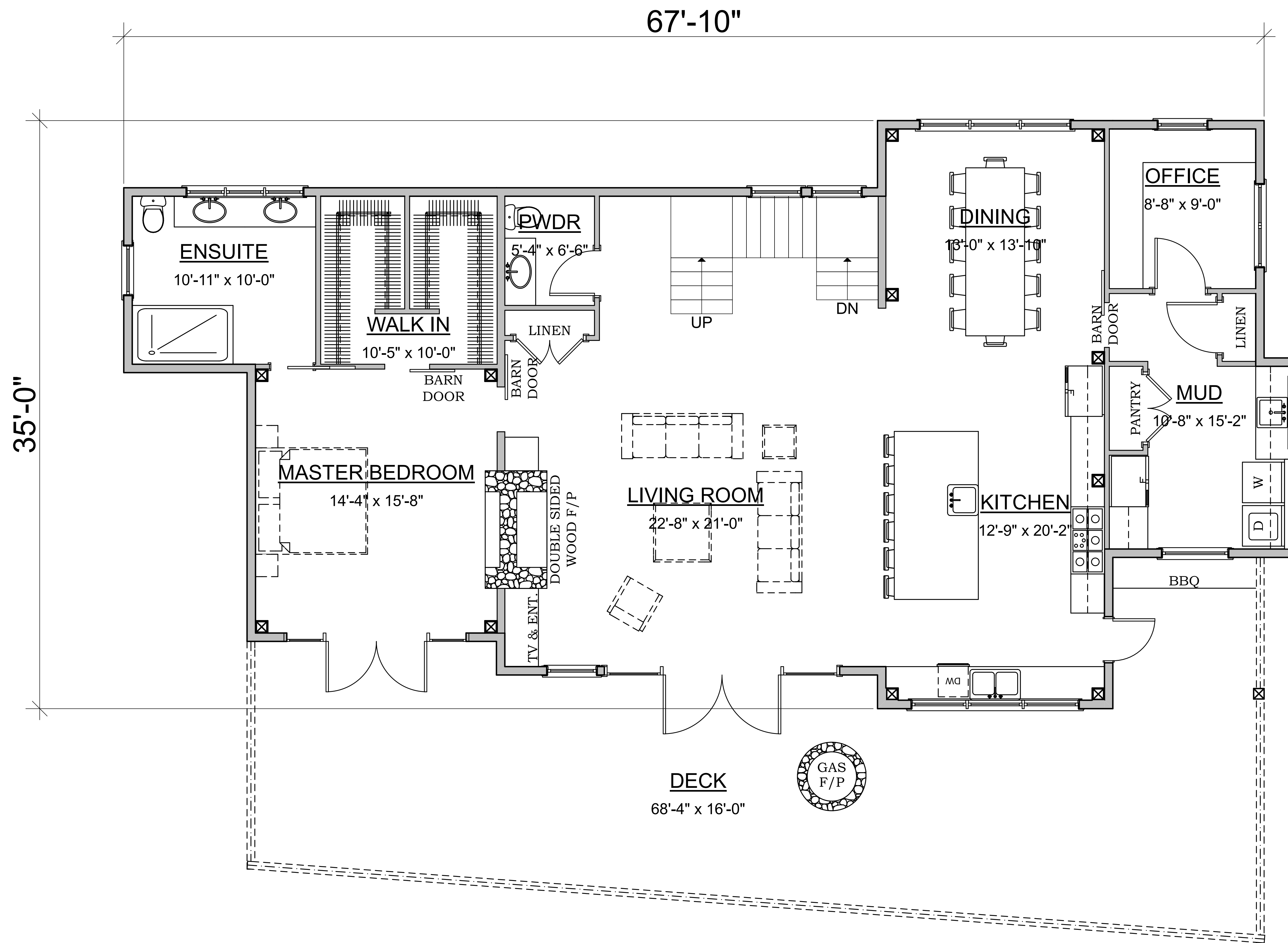
FIRST FLOOR PLAN AREA: 1,820 sq ft
